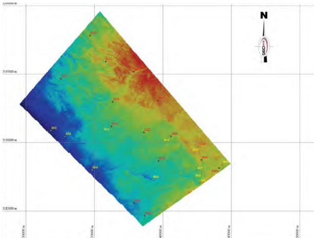
Multibeam bathymetry with positions seabed ground-truth
