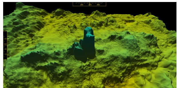
Details, multibeam and sidescan images of the shipwreck 'Driskos'
