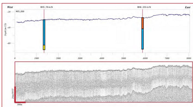
Multichannel seismic data
